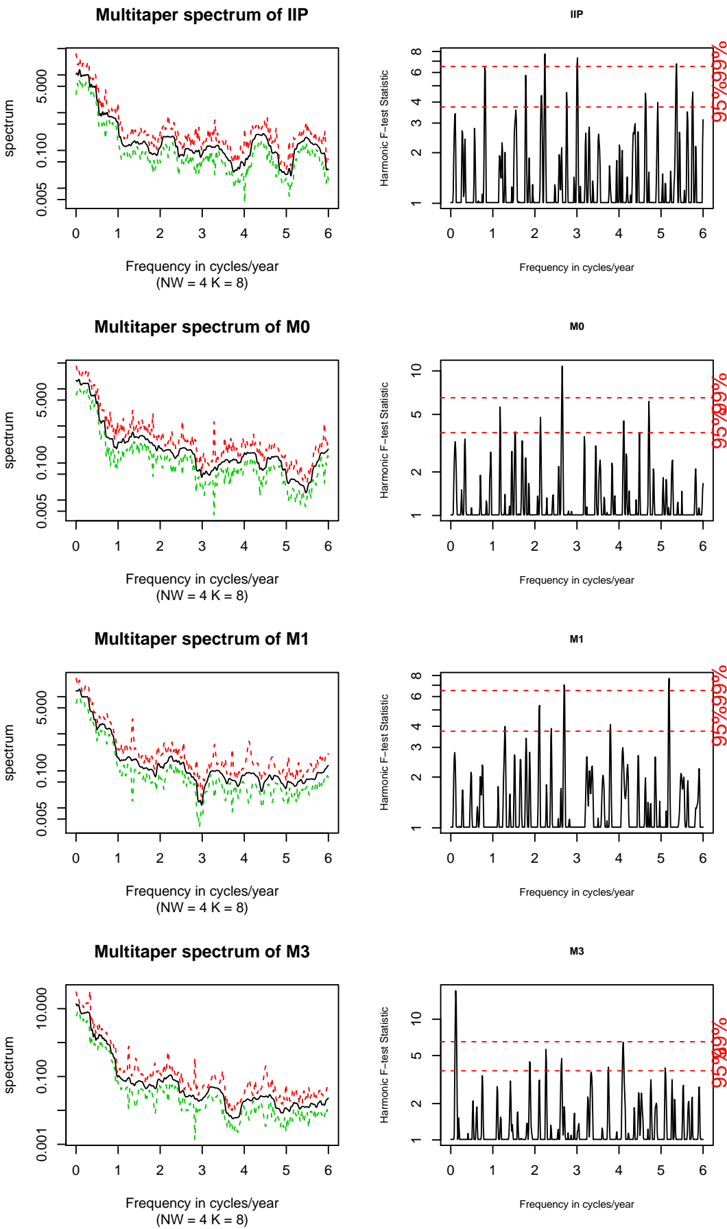
Figure 1: Multitaper Spectrum Estimates and Thompson F-statistics, nw = 4, k = 8
